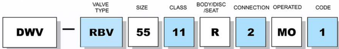
Selection Table of Butterfly Valves
